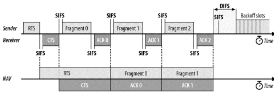
Figure 3-8. Fragmentation burst
