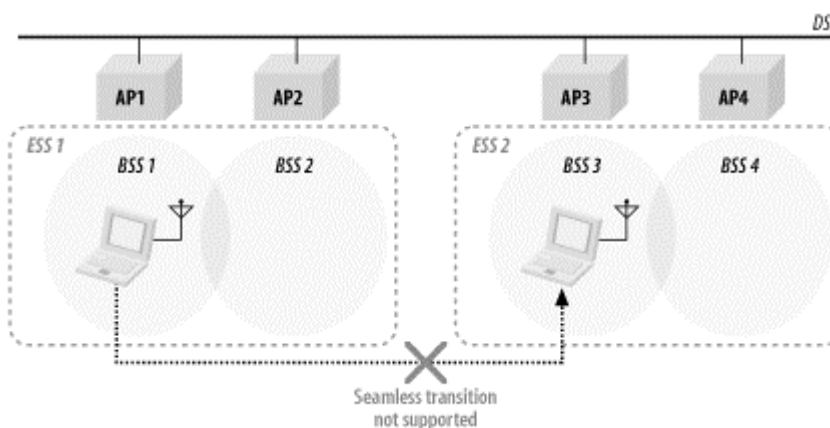
Figure 2-10. ESS transition
