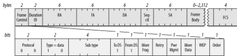
Figure 4-11. WDS frames
