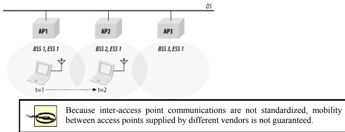
Figure 2-9. BSS transition
