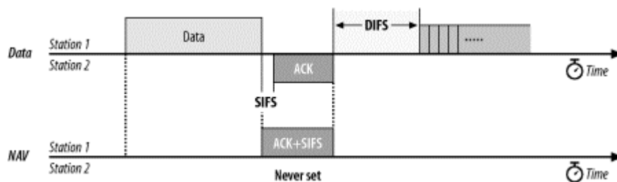
Figure 3-15. Basic positive acknowledgment of data
