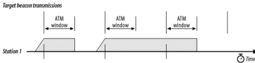
Figure 7-15. ATIM effects on power-saving modes
