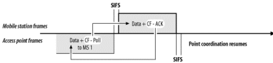
Figure 8-3. Data+CF-Ack usage
