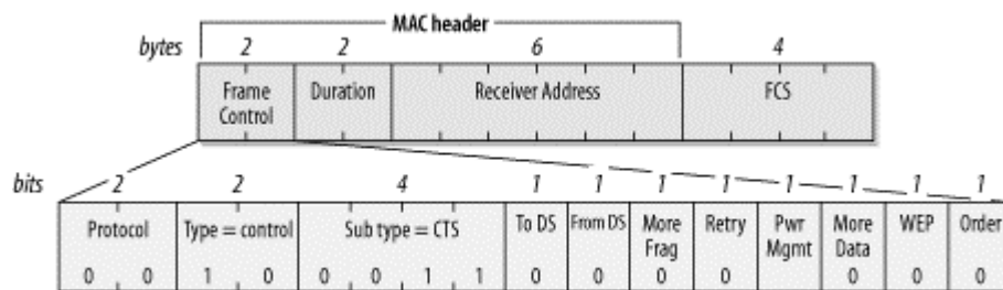
Figure 4-15. CTS frame
