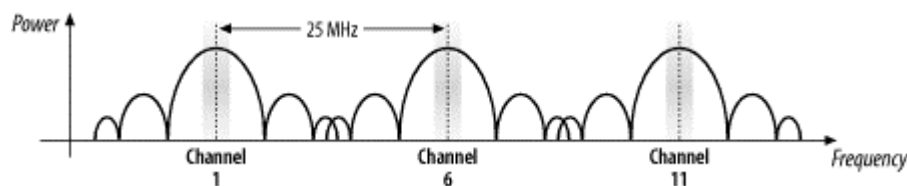
Figure 10-16. Channel separation in 802.11 DS networks
